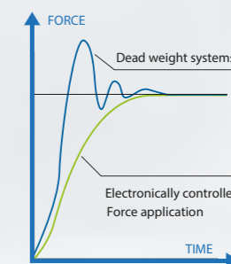
Load cell, closed loop, force feedback system
